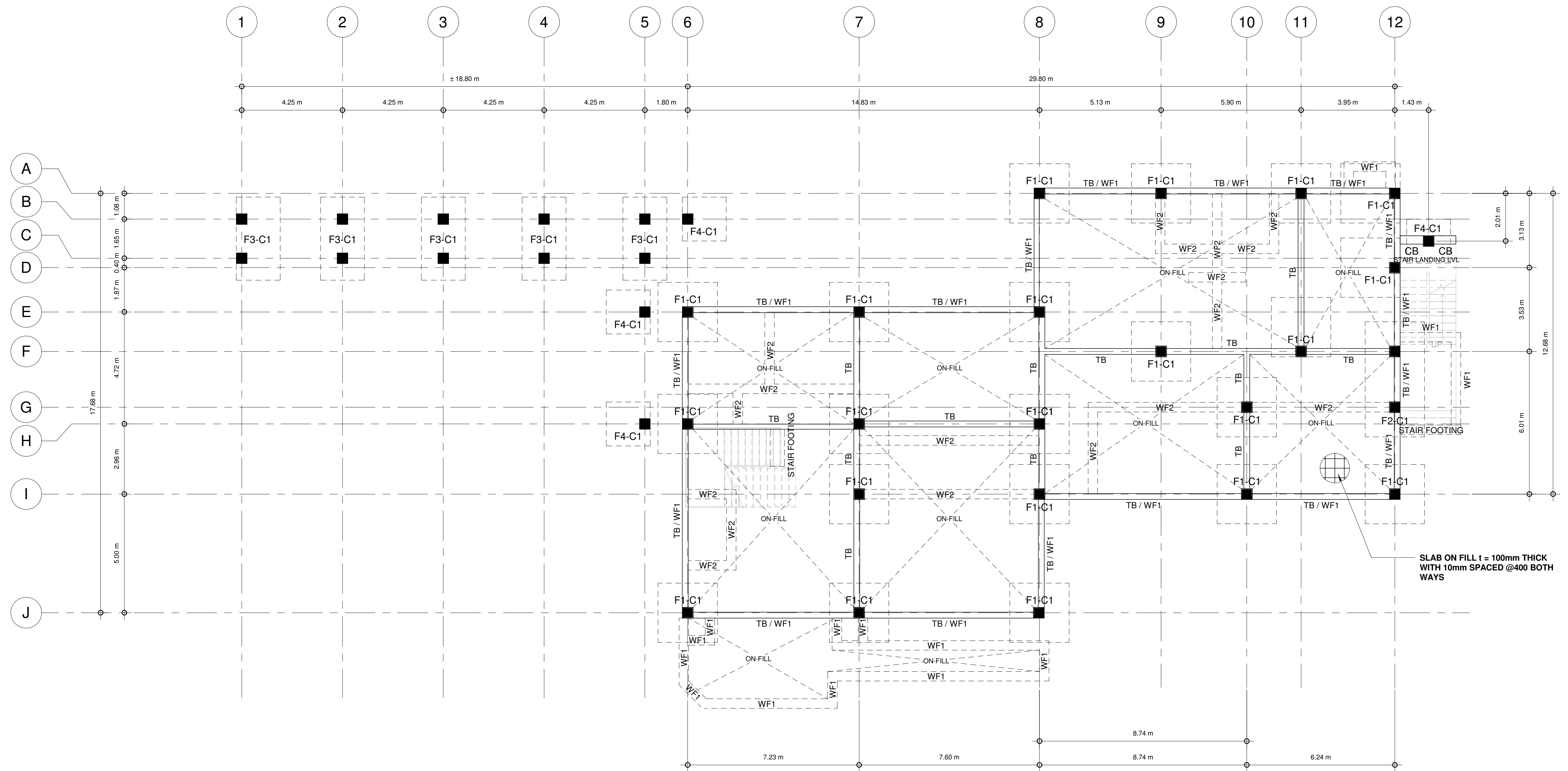
1 FOUNDATION PLAN 1 : 100 meters
